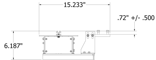
M10 LIGHTNING SHAKER ASSEMBLY
